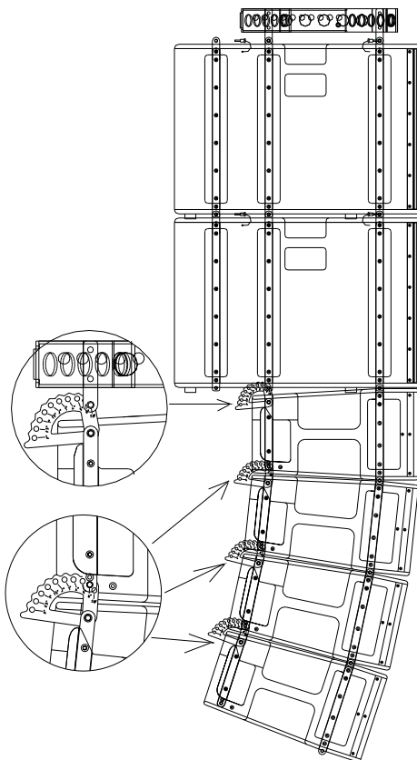
Fig.36. X210 + X215W Flying, curved Line Array
