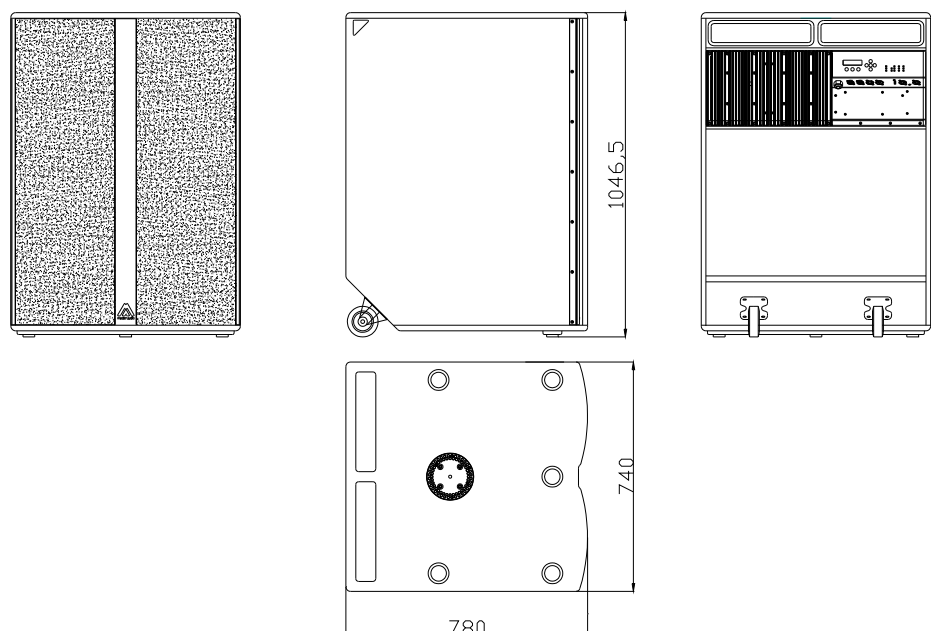
Fig.17. X218W3K cabinet. External dimensions
