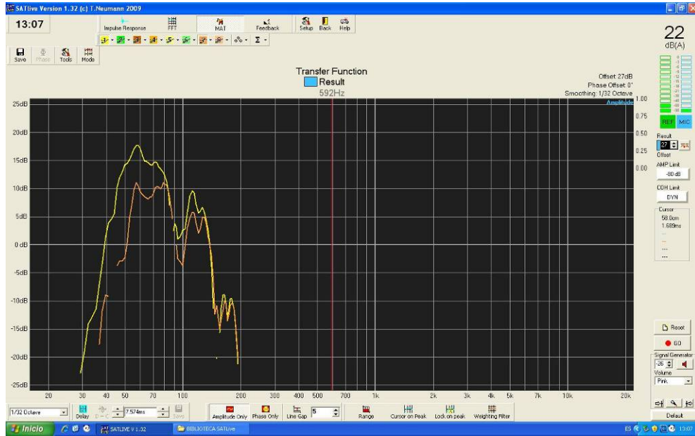
Fig.24b. X215W total back energy rejection. Yellow curve without central cardioid subwoofer; orange curve adding central cardioid subwoofer.
