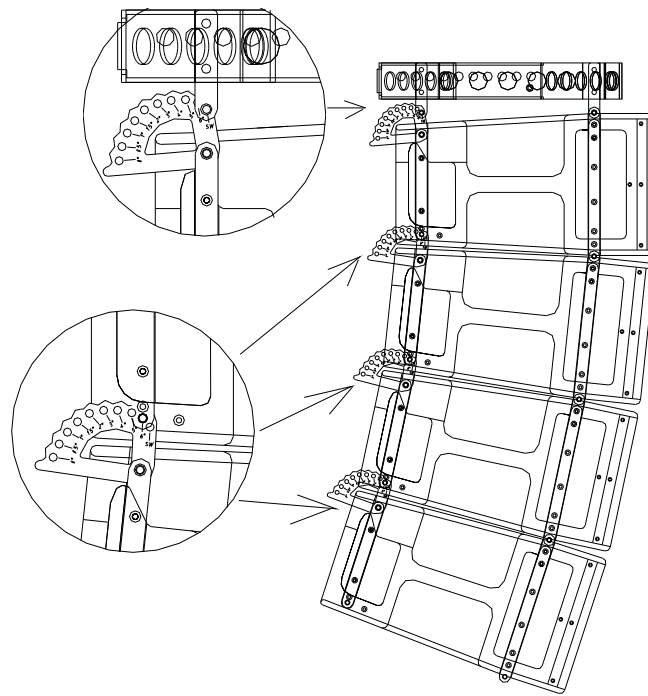
Fig.32. X210 Flying. 6° Curved Line Array (Cabinet 1 Back Guide = SW) (Cabinet 2/3/4 Back Guide = 6°)
