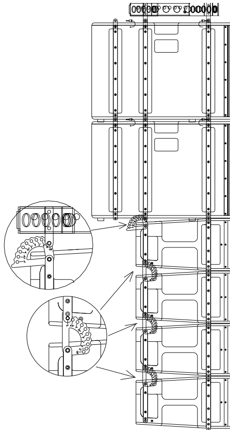
Fig.35. X210 + X215W flying, flat Line Array
