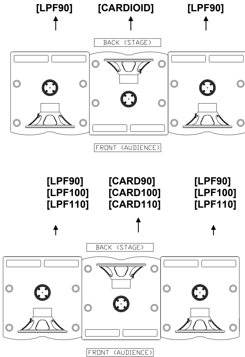
Fig.24. Presets for cardioid configuration
