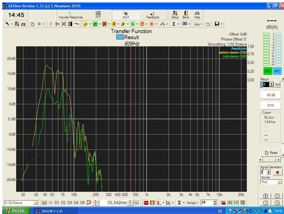
Fig.24c. X218W total back energy rejection. Yellow curve without central cardioid subwoofer; green curve adding central cardioid subwoofer.
