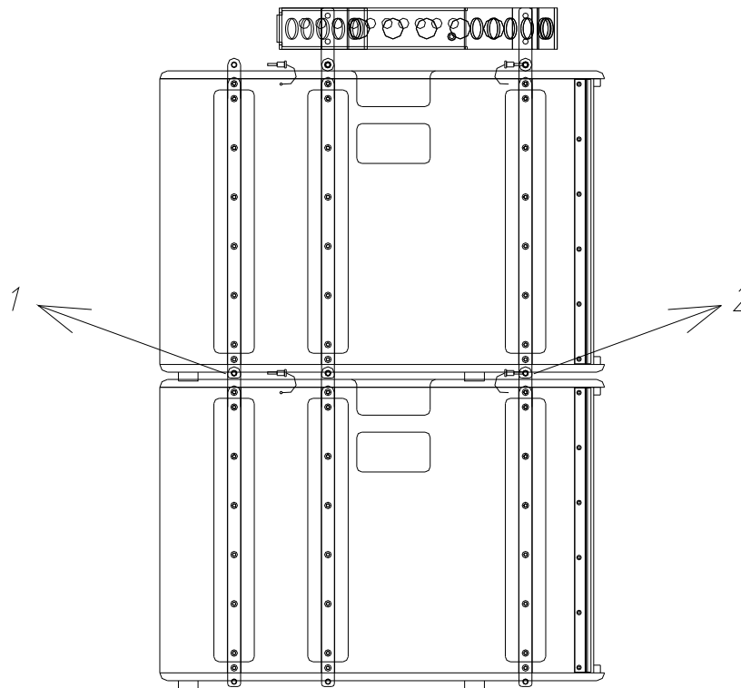
Fig.33. X215W Flying, two units
