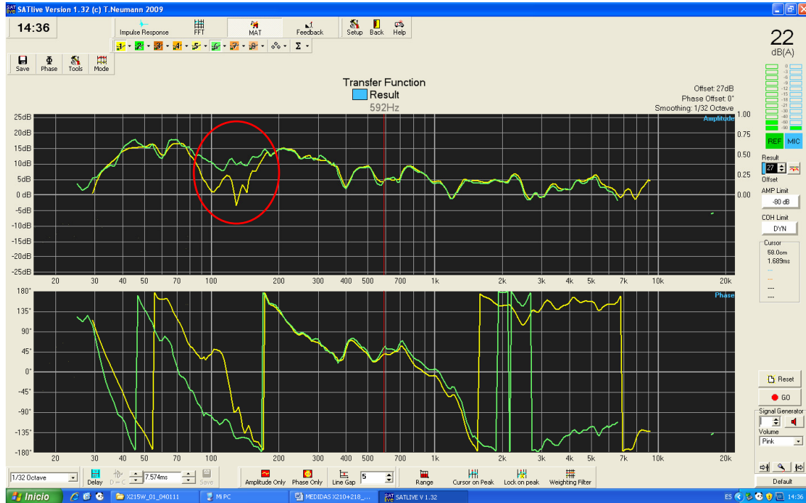
Fig.39. Magnitude and phase response of the complete aligned system (with delay), green curve
