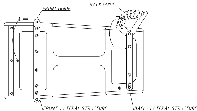
Fig.26. Flying hardware (lateral view)
