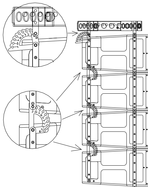
Fig.31. X210 Flying. Flat Line Array
