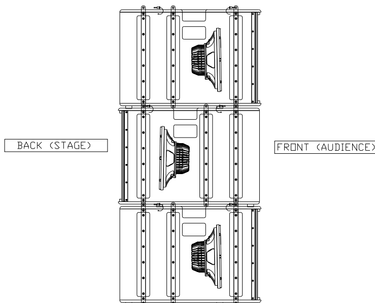
Fig.22. Cardioid configuration for X215W subwoofer
