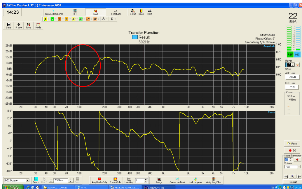
Fig.38. Magnitude and phase response of the complete unaligned system (with no delay)
