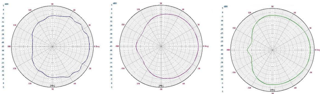
Fig.24a. Back energy rejection at 40Hz / 50 Hz / 63Hz
