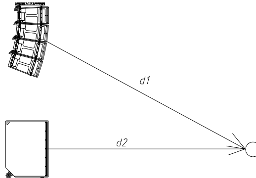
Fig.37. This system is not completely aligned because d_1 and d_2 are not equal.
