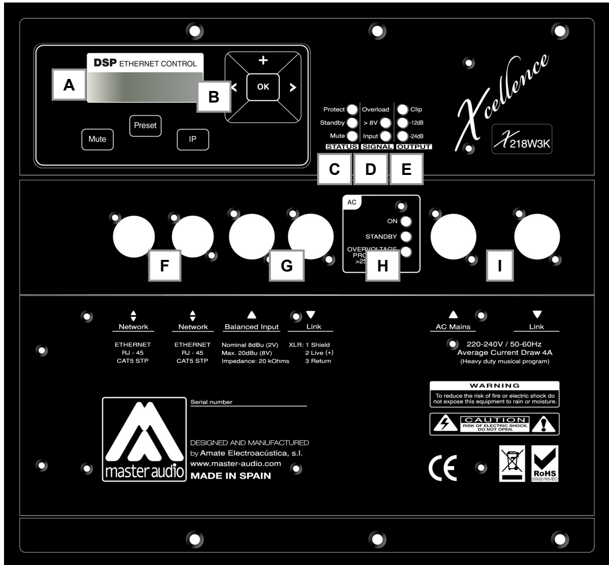
Fig.19. X218W3K connection panel
