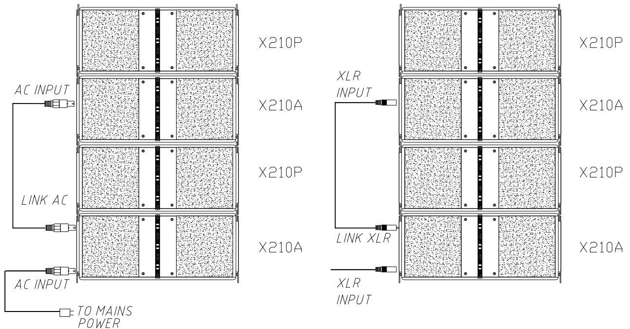
Fig.25. Parallel connection for the Xcellence Line Array series (signal and mains)
