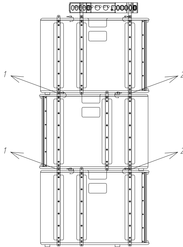
Fig.34. X215W Flying, three units in cardioid configuration
