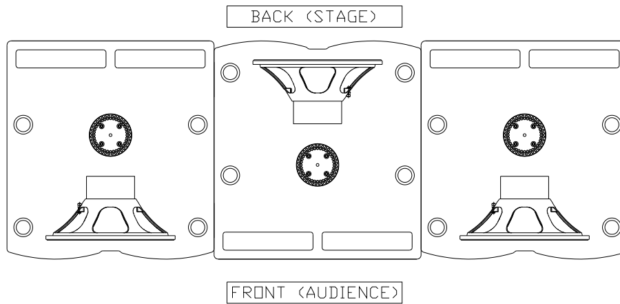
Fig.23. Cardioid configuration for X218W/X218W3K subwoofer
