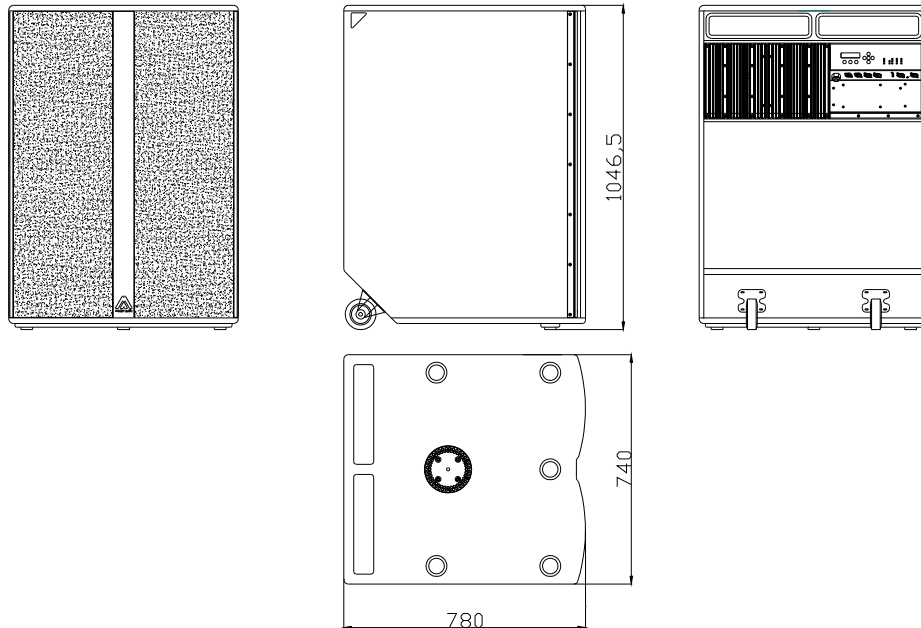
Fig.14. X218W cabinet. External dimensions
