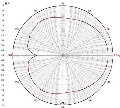
Fig.21. Cardioid pattern
